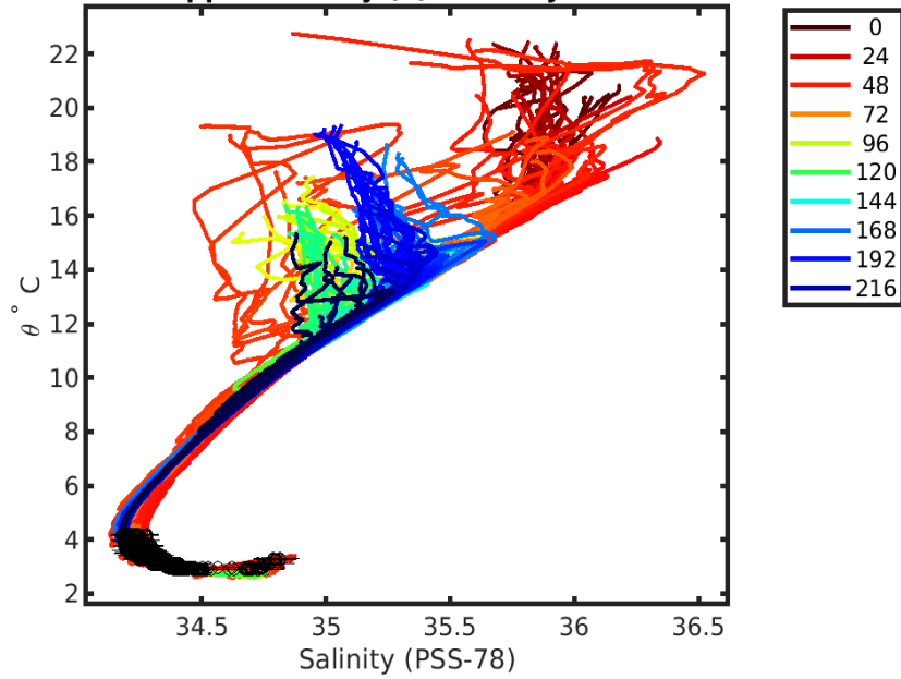
1901617 uncalibrated float data (-) and mapped salinity (o) with objective errors
