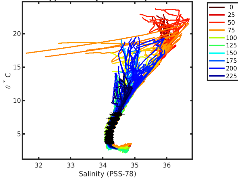
1901616 uncalibrated float data (-) and mapped salinity (o) with objective errors
