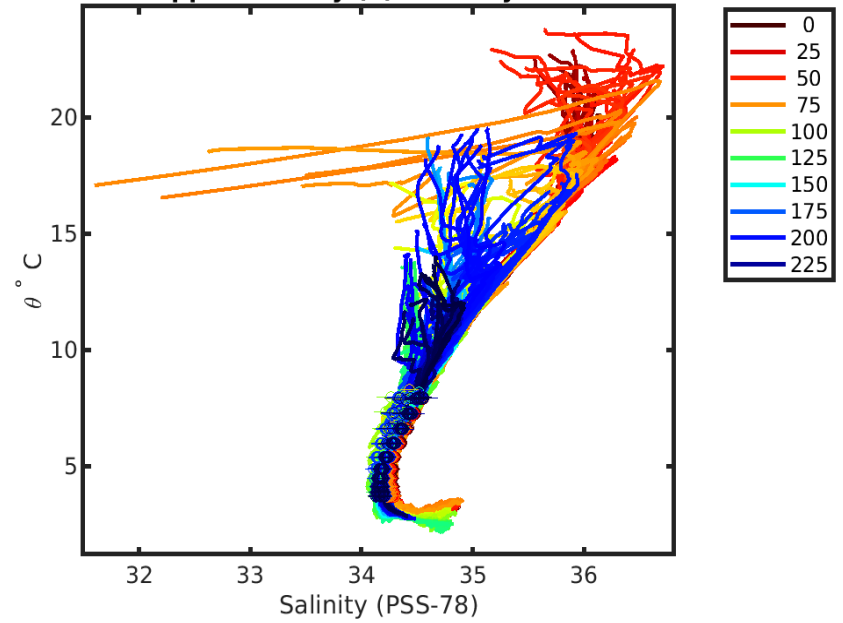
1901616 calibrated float data (-) and mapped salinity (o) with objective errors
