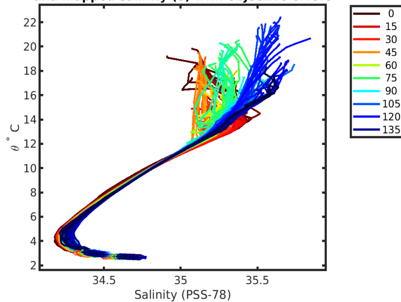
1901577 calibrated float data (-) and mapped salinity (o) with objective errors
