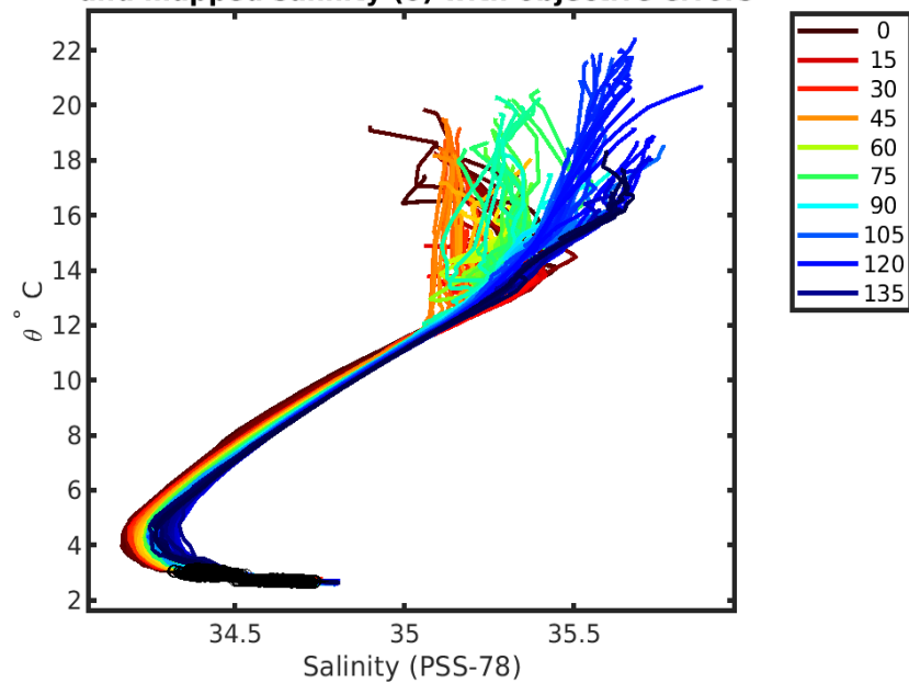
1901577 uncalibrated float data (-) and mapped salinity (o) with objective errors
