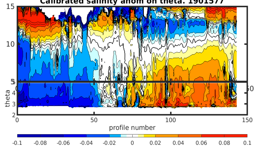
Calibrated salinity anom on theta. 1901577
