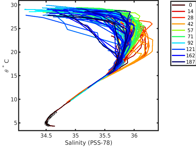
1900528 uncalibrated float data (-) and mapped salinity (o) with objective errors
