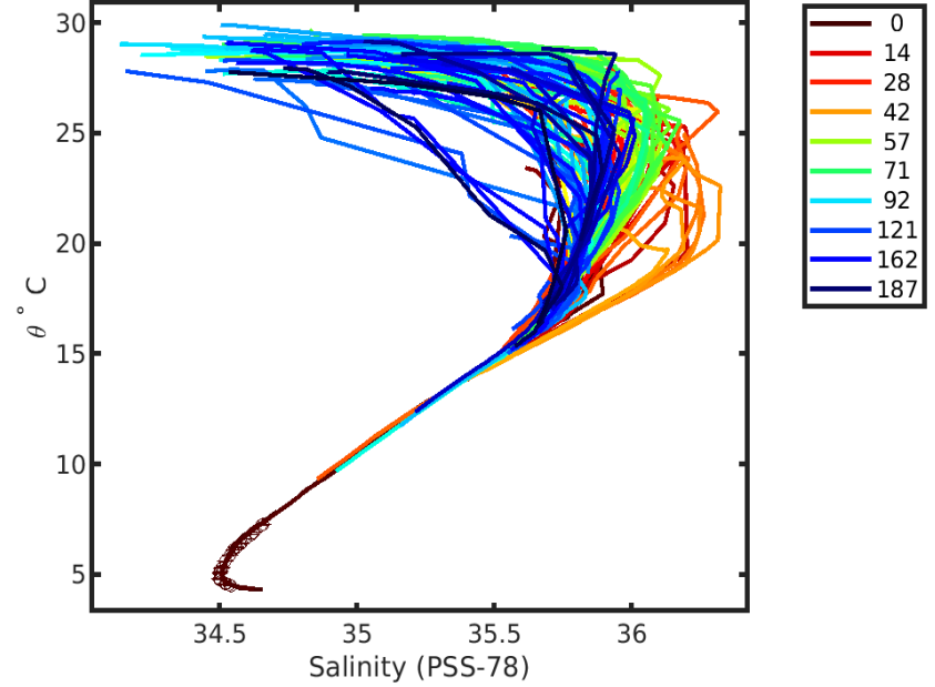
1900528 calibrated float data (-) and mapped salinity (o) with objective errors
